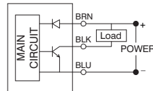
Hall-NPN effect (3 wires)
