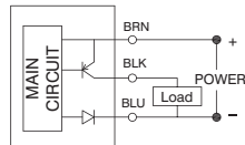
Hall-PNP effect (3 wires)
