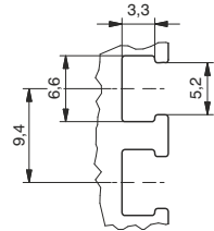
Sensor slot detail type "B" (n° 6 slots)
